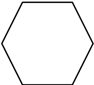
hexagon
