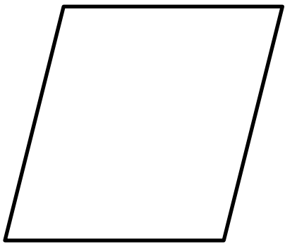
parallelogram
